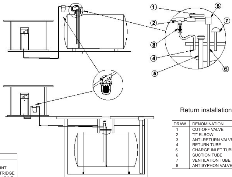
Right filter installation in over and underground tanks
